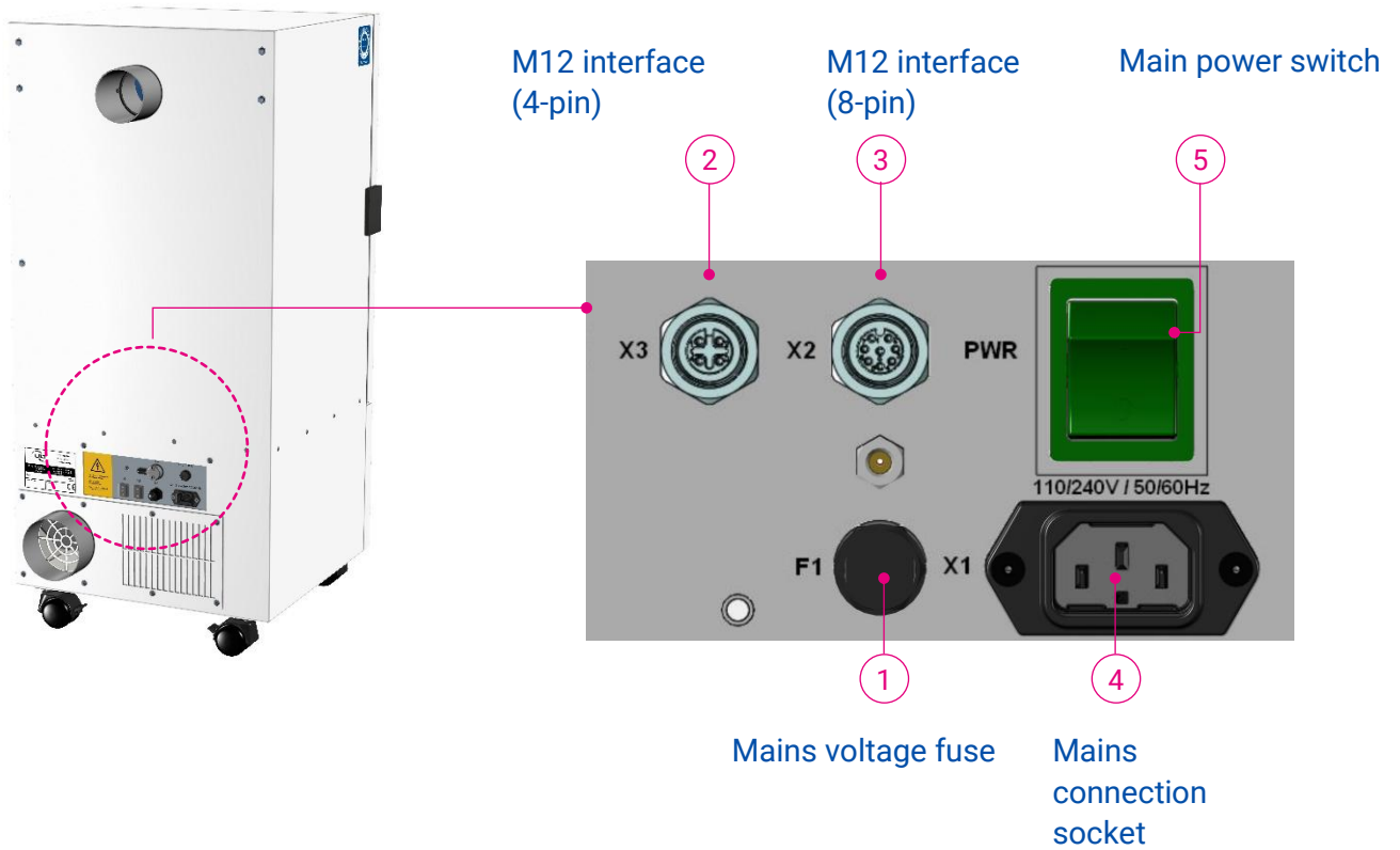
Figure 2: Rear interfaces of the ULT ProSight control
