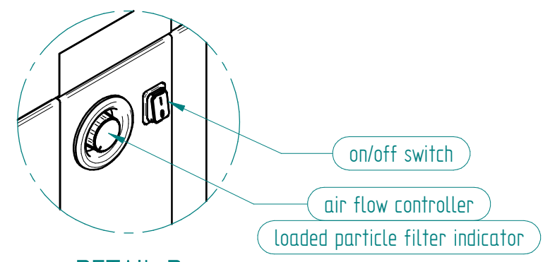
DETAIL D
